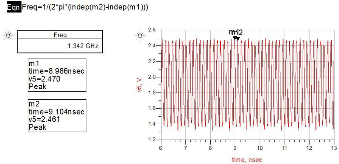
Figure 32. Transient response of Ring VCO
