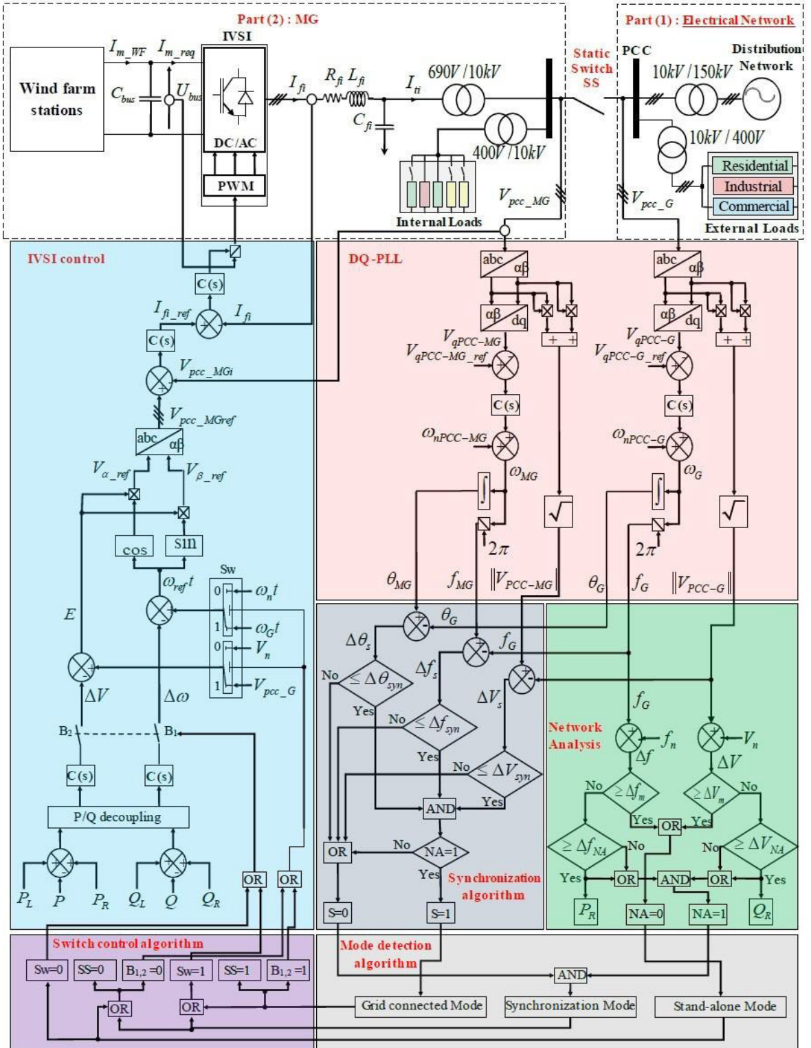
Figure 41. Block Diagram of the proposed synchronization method [20]
