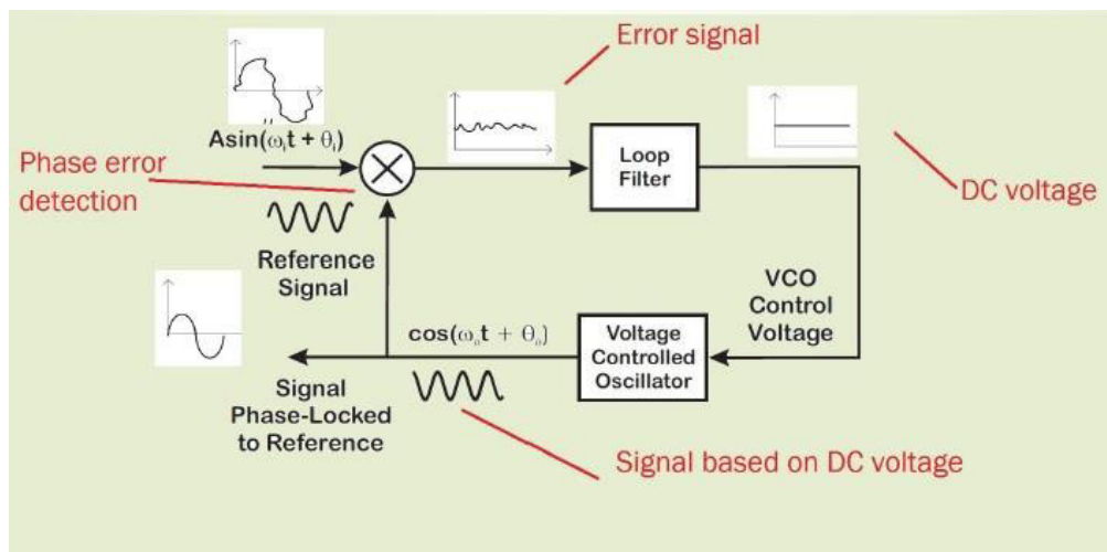
Figure 28. Signal processing in PLL [16]
