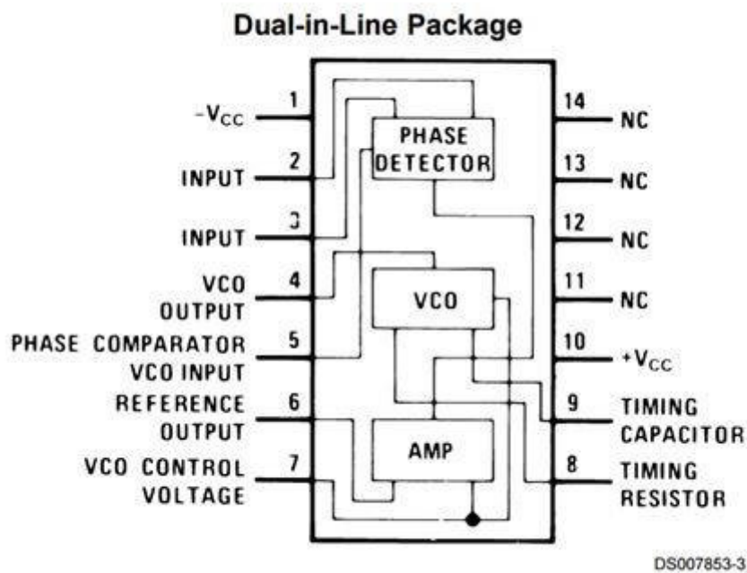
44. NE565 PLL Pin Diagram [25]
