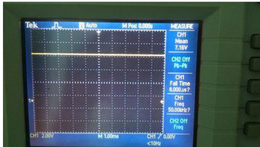
Figure 52. Pin 7 wave in 1.121 kHz
