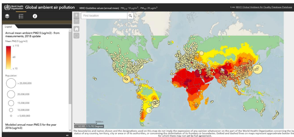
Εικόνα 3: Annual mean ambient PM 2.5 (µg/m 3 ) - from measurements, 2018 update (WHO)
