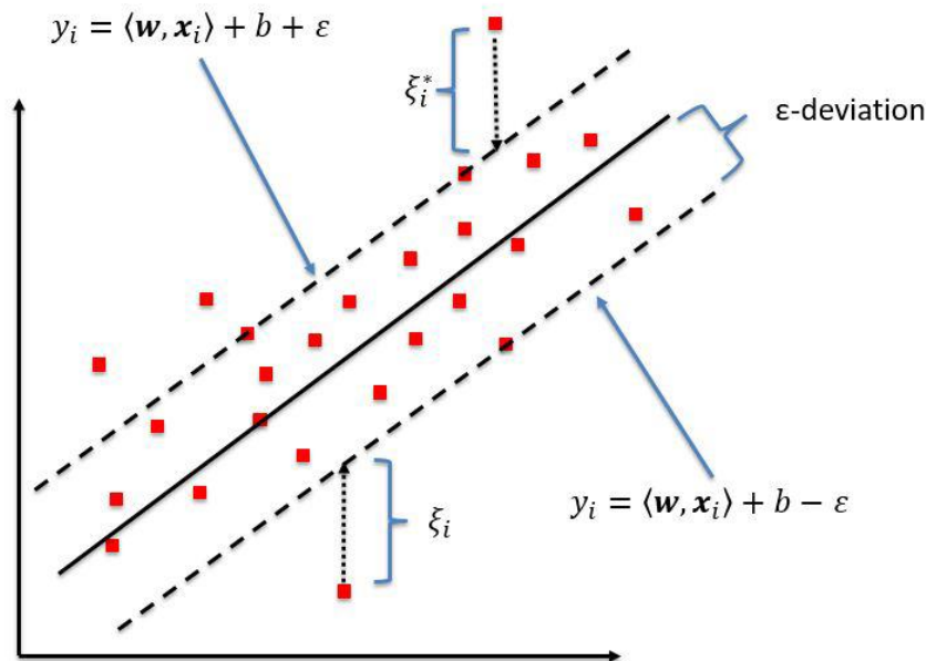
Εικόνα 15: https://www.researchgate.net/figure/Schematic-of-the-one-dimensional-support-vector-regression-SVR-model-Only-the-points_fig5_320916953 [26]
